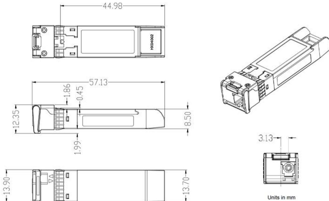
Figure2. Mechanical Outline
